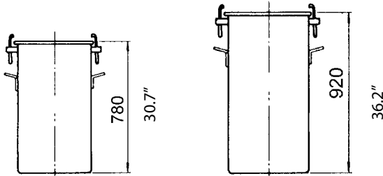
7066 Steel Container 90 l/23.8 gal.
